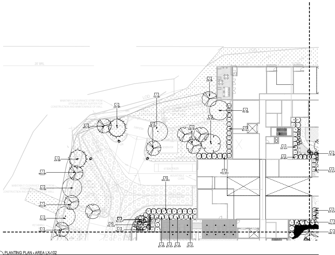
PLANTING PLAN - AREA LX-102 SHEET 1 OF 1
