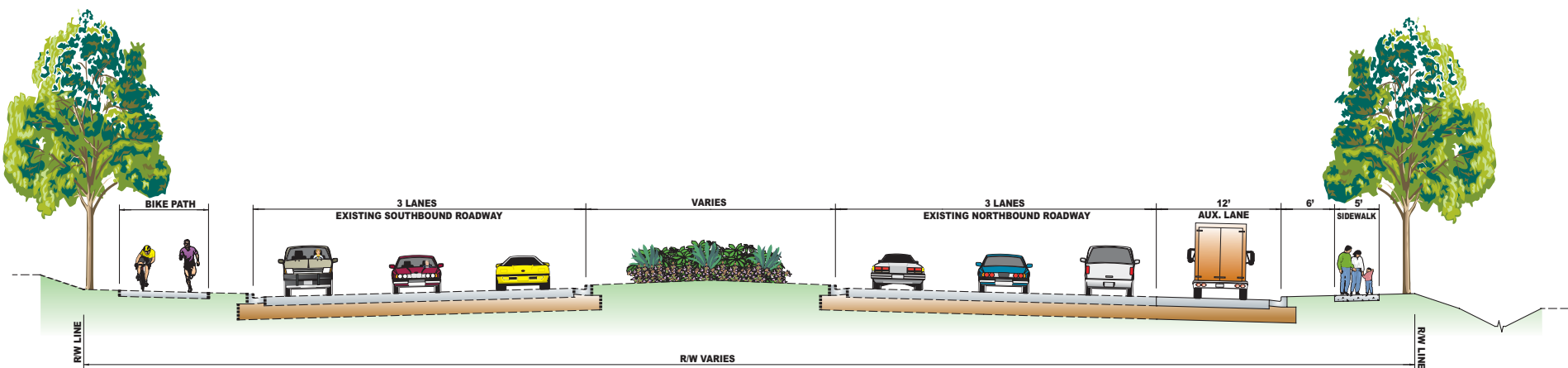
MD 355 TYPICAL SECTION FROM CHRISTOPHER AVE. TO WATKINS MILL ROAD
