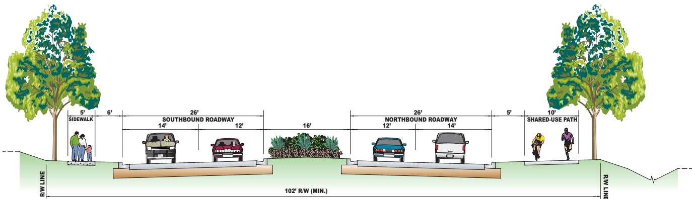
WATKINS MILL ROAD / MIDCOUNTY HIGHWAY TYPICAL SECTION FROM MD 355 TO RIDGE ROAD (MD 27)
