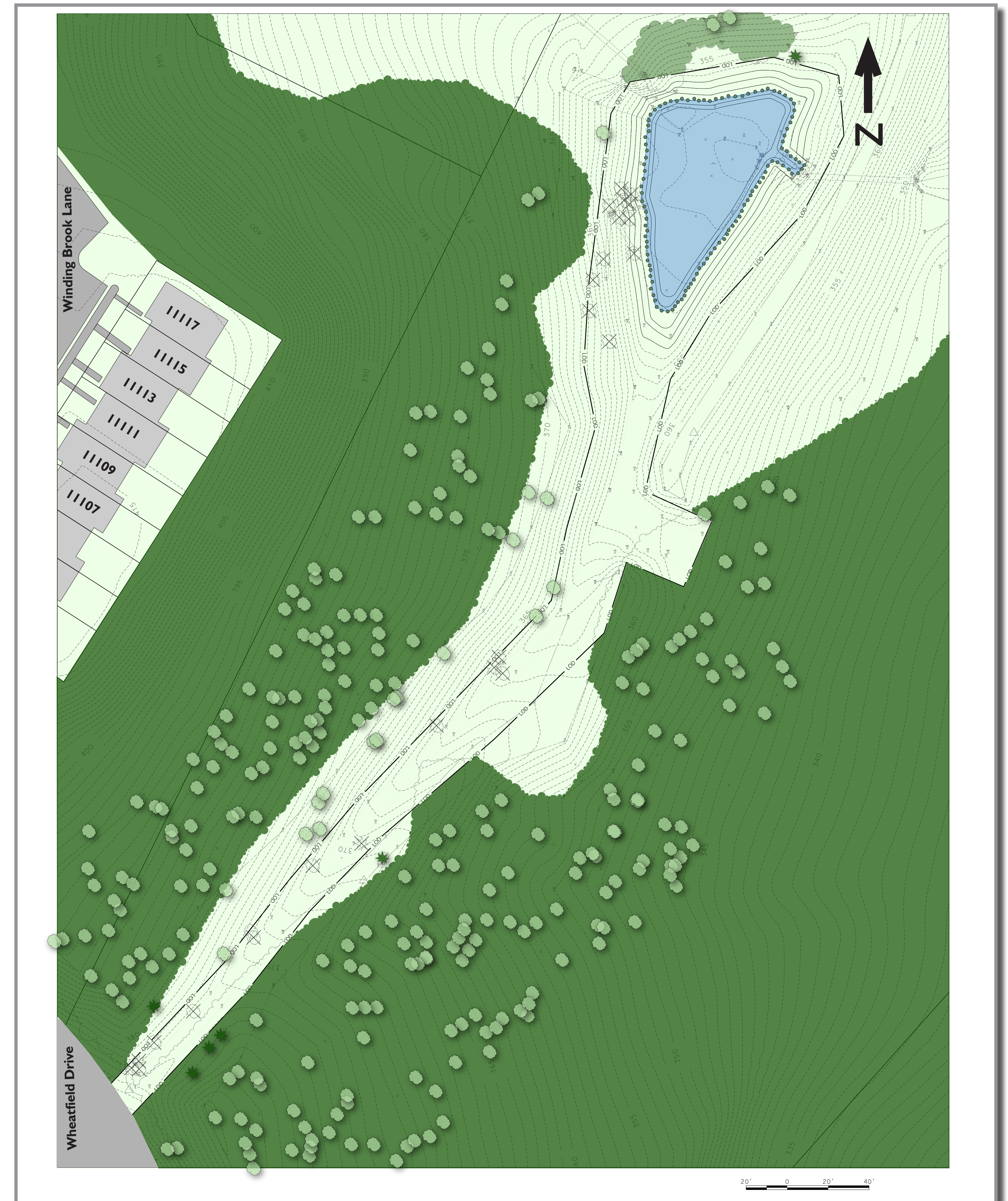
Construction Access Map
