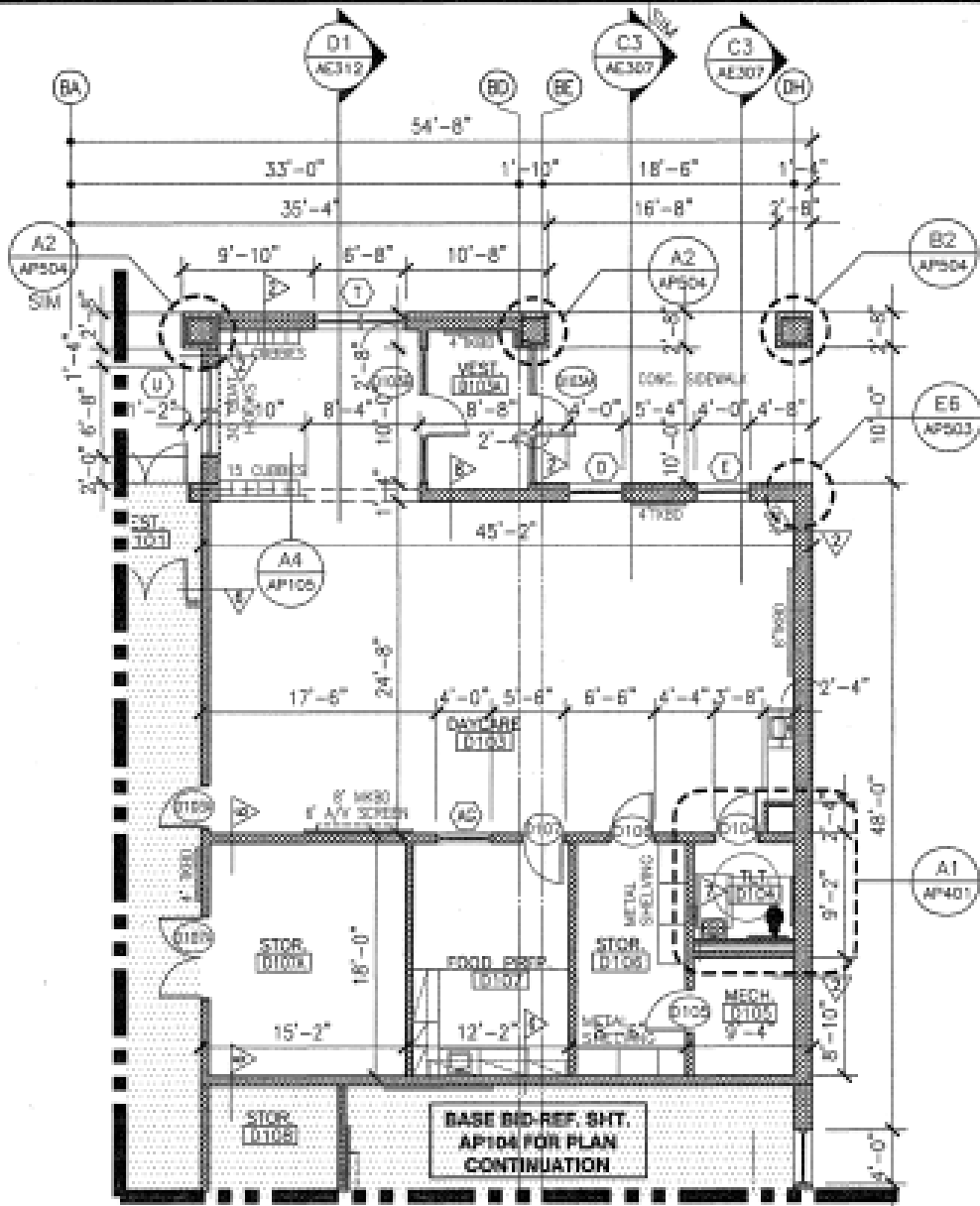
D3 1st FLOOR PLAN - AREA 'D' ADD ALT. #2A/2B 1/8" = 1'-0"
