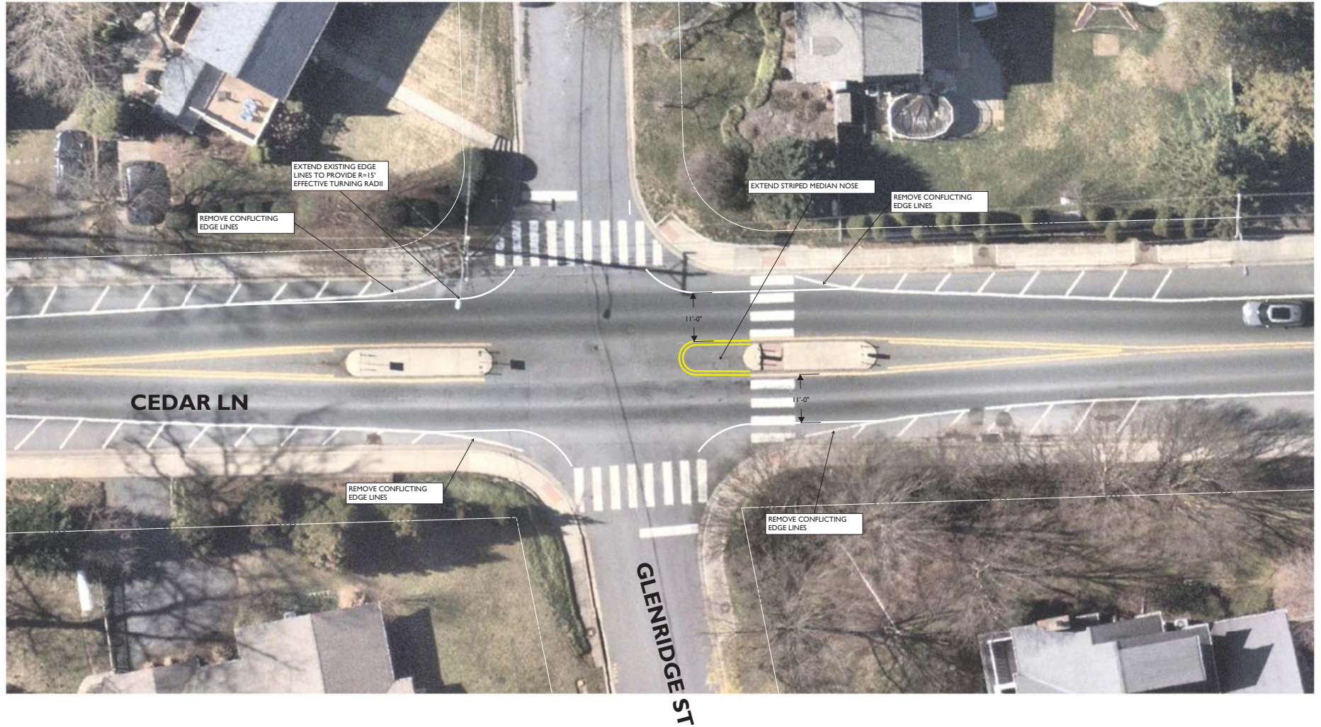
CEDAR LN AT GLENRIDGE ST STRIPING MODIFICATIONS
