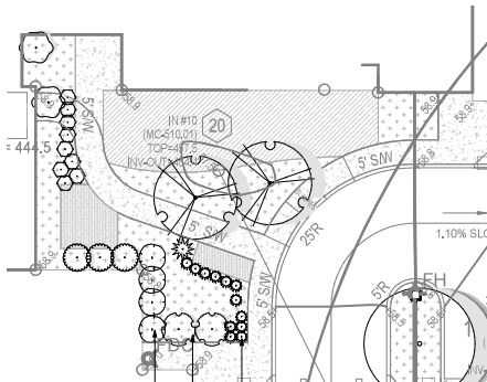
3. FITNESS GREEN PLANTING PLAN 1" = 10'-0"
