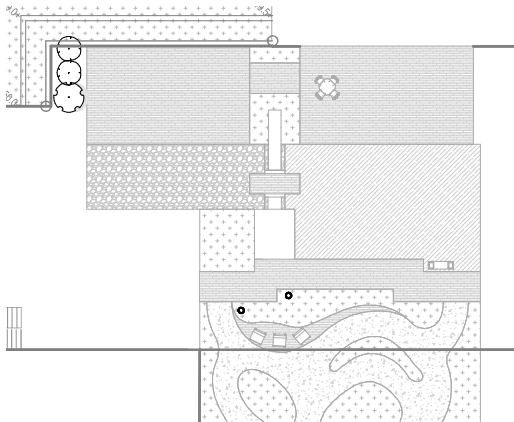
1. AL GARDEN COURTYARD PLANTING PLAN 1" = 10'-0"
