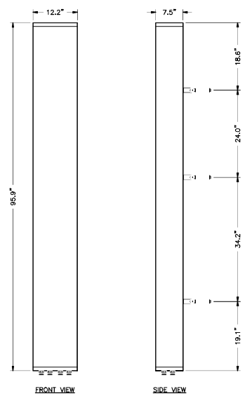
3 MX06FHG865-HG ANTENNA DETAILS A-1 NTS
