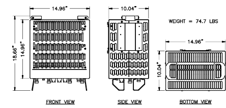
4 SAMSUNG B2/B66A RRH ORAN RF4439d-25A A-2 NTS
