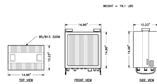
5 B5/B13 RF4461D-13A RRH (REMOTE RADIO HEAD) A-1 NTS
