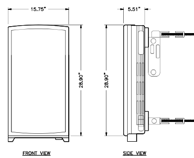
2 MT6413-77A INTEGRATED ANTENNA A-1 NTS
