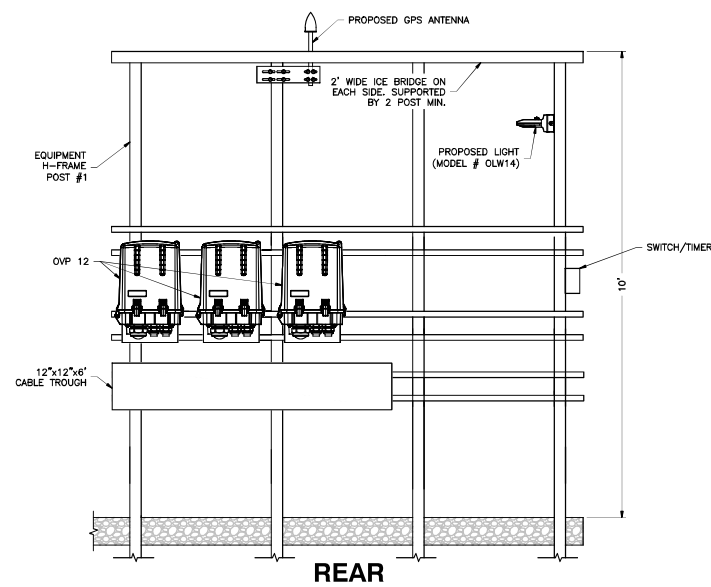
1 H-FRAME RISER DETAILS A-2 NTS
