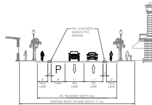
PROPOSED 13TH STREET MID-BLOCK
