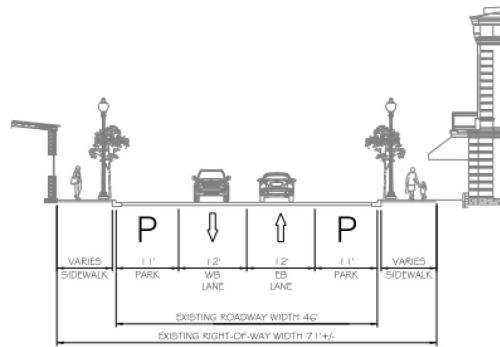
EXISTING 13TH STREET MID-BLOCK
