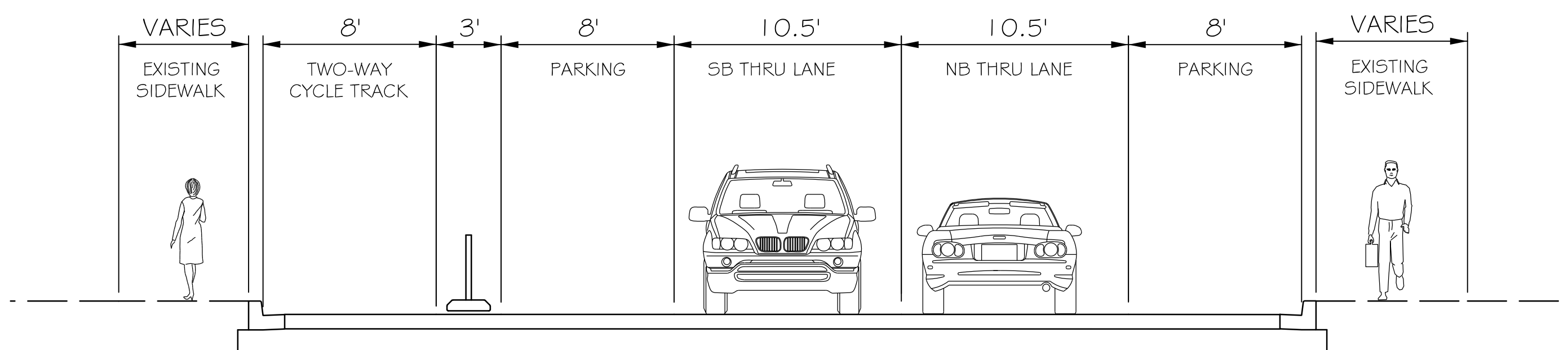
REEDIE DRIVE TO SOUTH OF UNIVERSITY BOULEVARD (MD 193) PROPOSED TYPICAL SECTION
