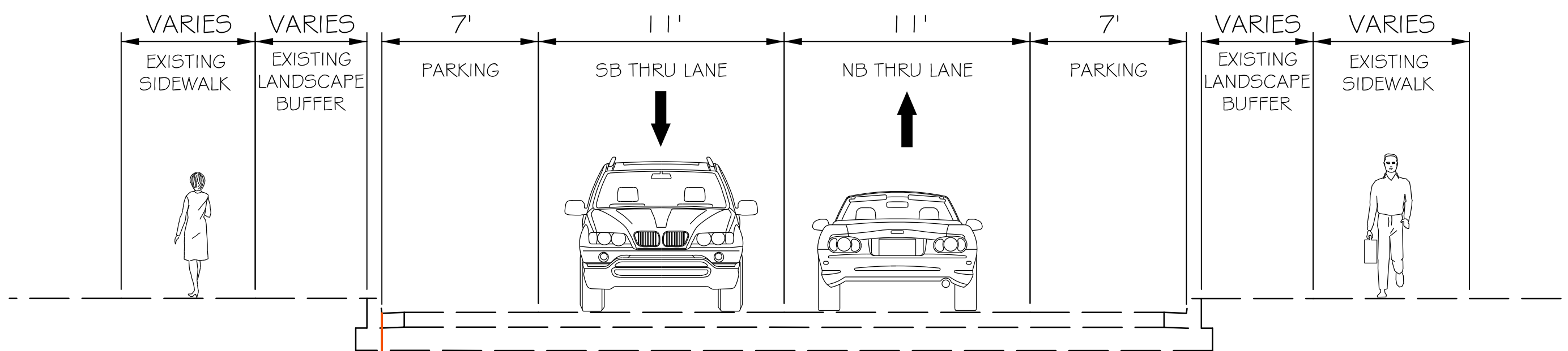
BLUERIDGE AVENUE TO ARCOLA AVENUE EXISTING TYPICAL SECTION
