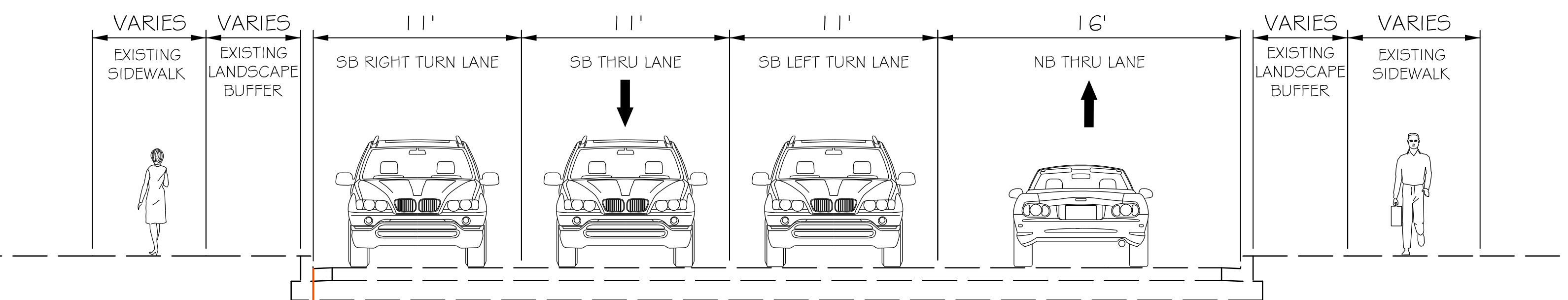
UNIVERSITY BOULEVARD (MD 193) EXISTING TYPICAL SECTION
