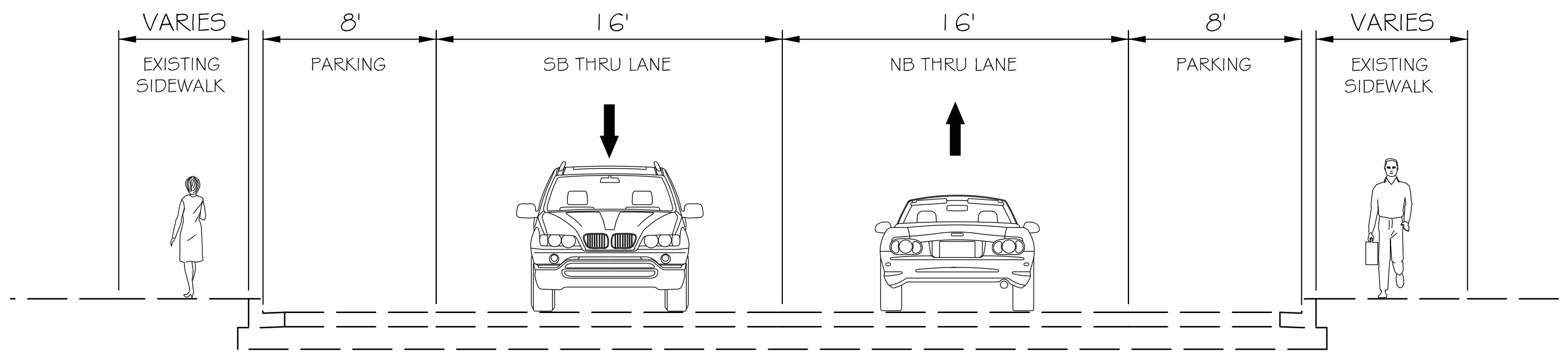
NORTH OF UNIVERSITY BOULEVARD (MD 193) TO BLUERIDGE AVENUE EXISTING TYPICAL SECTION
