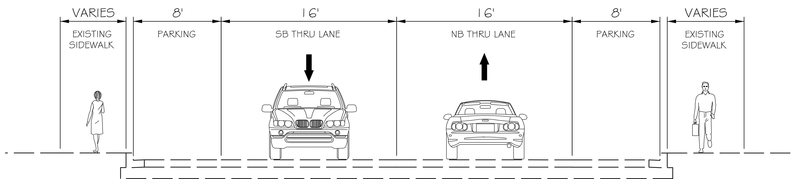
REEDIE DRIVE TO SOUTH OF UNIVERSITY BOULEVARD (MD 193) EXISTING TYPICAL SECTION
