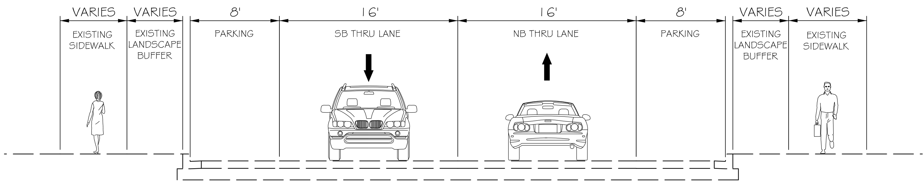
WINDHAM LANE TO PRITCHARD ROAD EXISTING TYPICAL SECTION
