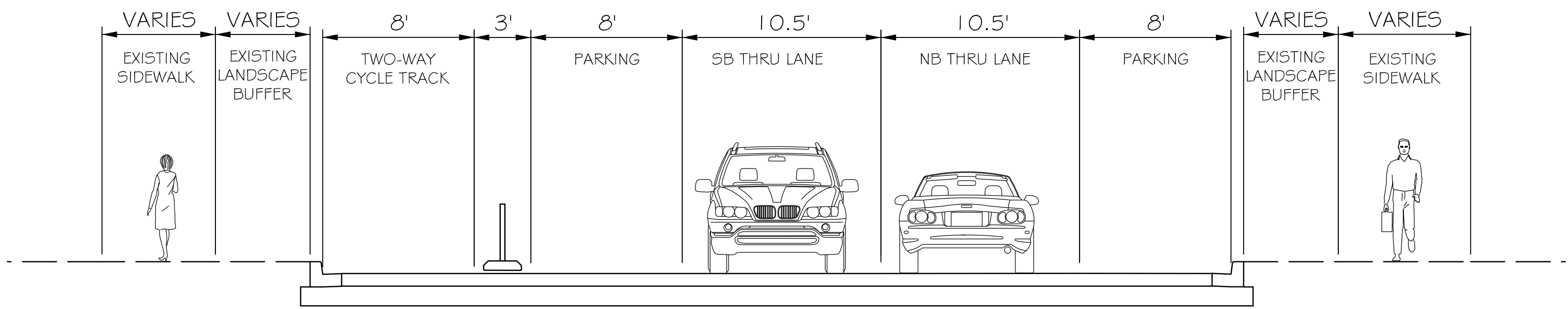
WINDHAM LANE TO PRITCHARD ROAD PROPOSED TYPICAL SECTION
