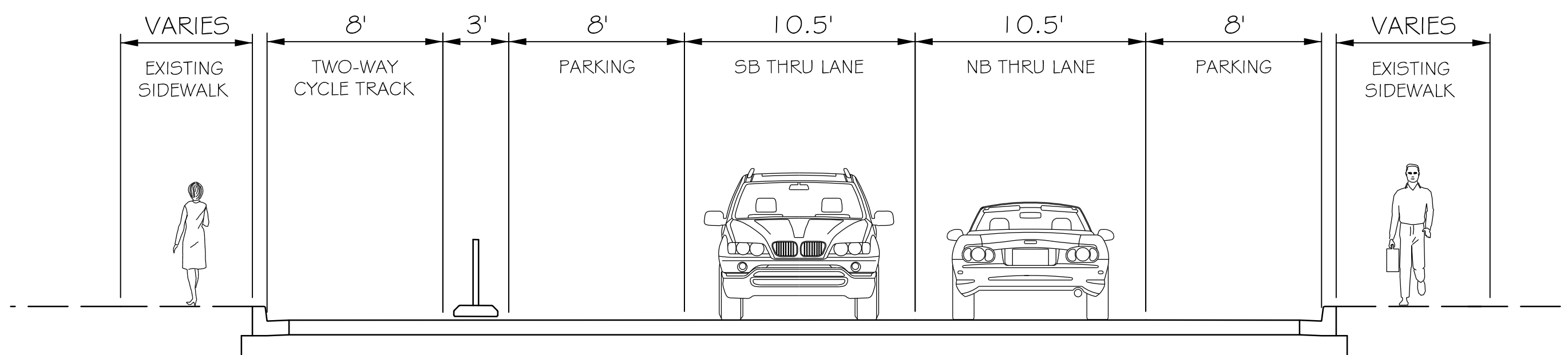
NORTH OF UNIVERSITY BOULEVARD (MD 193) TO BLUERIDGE AVENUE PROPOSED TYPICAL SECTION
