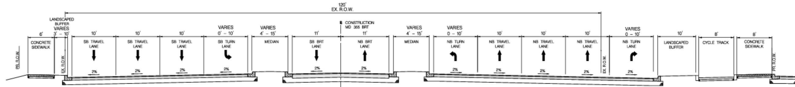
TYPICAL SECTION SEGMENT 2 TWO MEDIAN BRT LANES
