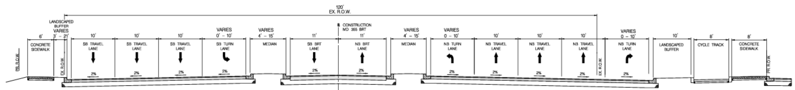
TYPICAL SECTION SEGMENT 2 TWO MEDIAN BRT LANES
