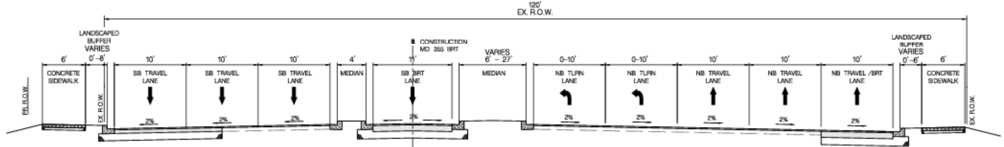
TYPICAL SECTION SEGMENT 2 - SEGMENT 3 ONE MEDIAN BRT LANE
