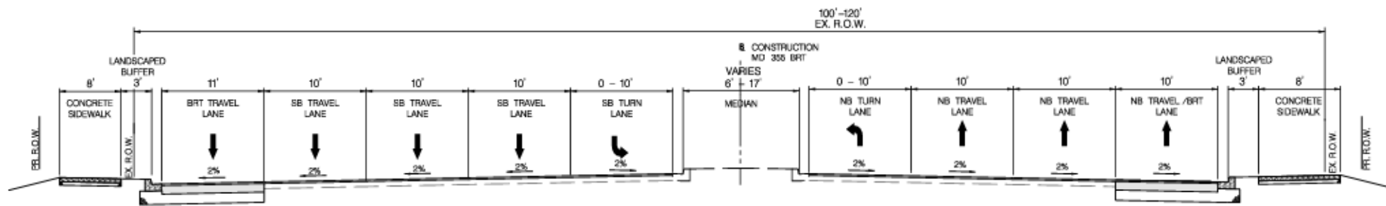
TYPICAL SECTION SEGMENT 3 MIXED TRAFFIC
