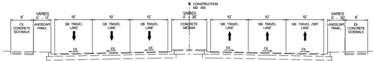
TYPICAL SECTION SEGMENT 5 MIXED TRAFFIC
