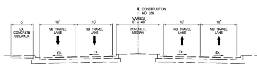
TYPICAL SECTION SEGMENT 5 MIXED TRAFFIC
