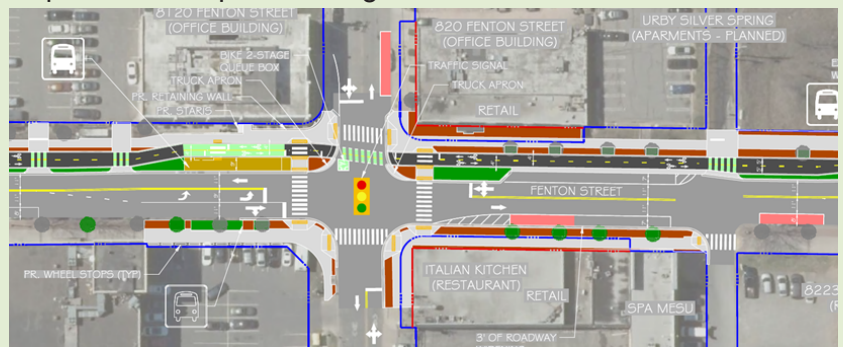
Excerpt of map of 65% Design of Fenton Street Cycletrack
