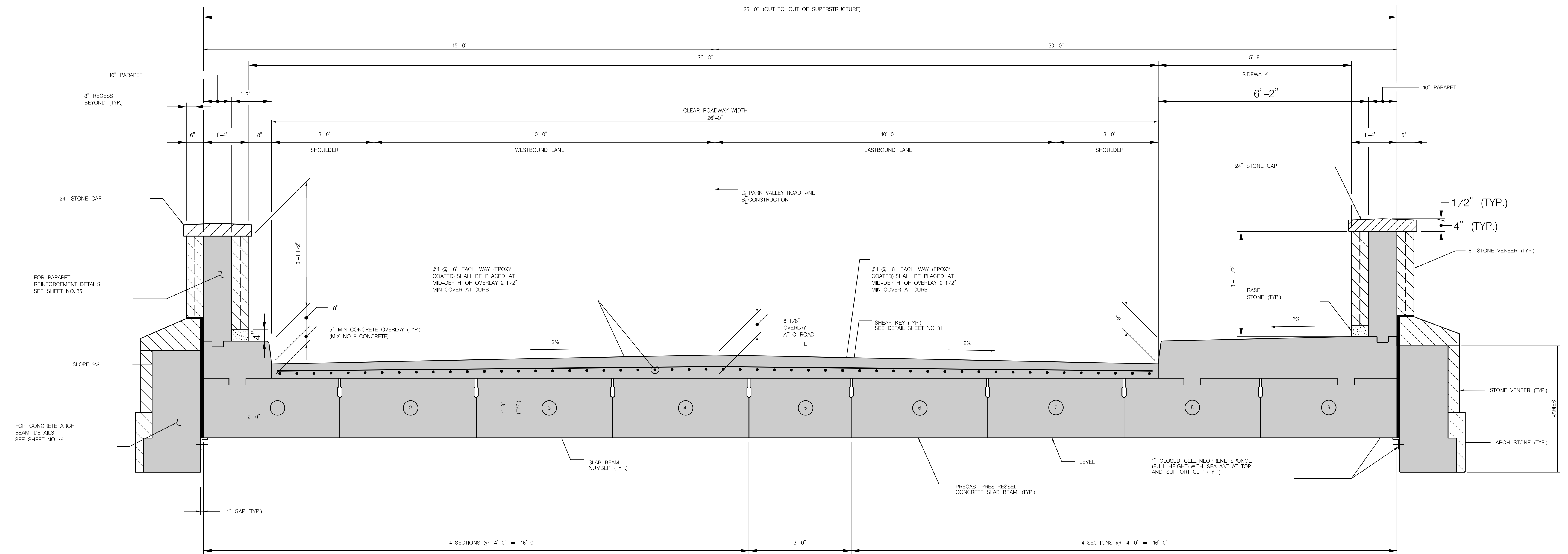
PROPOSED BRIDGE TYPICAL SECTION (LOOKING EAST)
