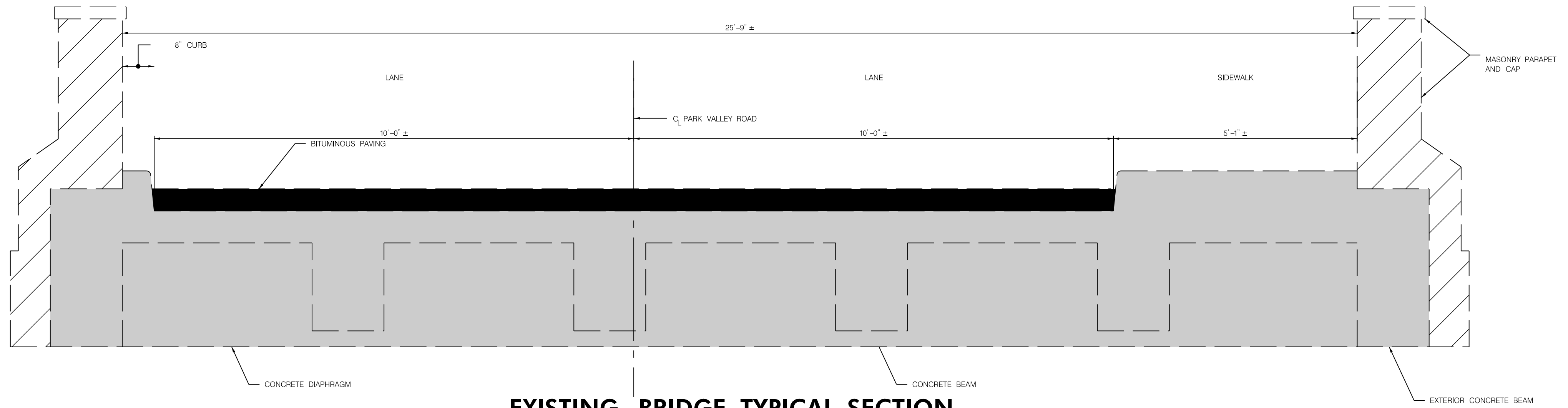
EXISTING BRIDGE TYPICAL SECTION (LOOKING EAST)
