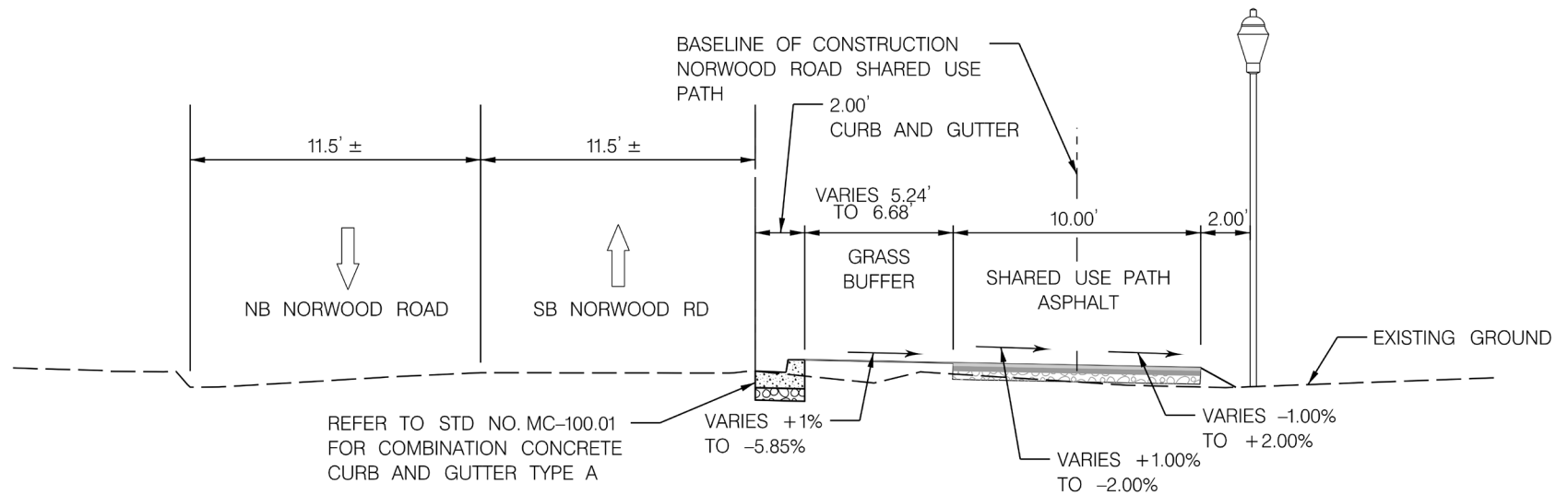
NORWOOD ROAD SHARED USE PATH TYPICAL SECTION ASPHALT PATH WITH CURB AND GUTTER
